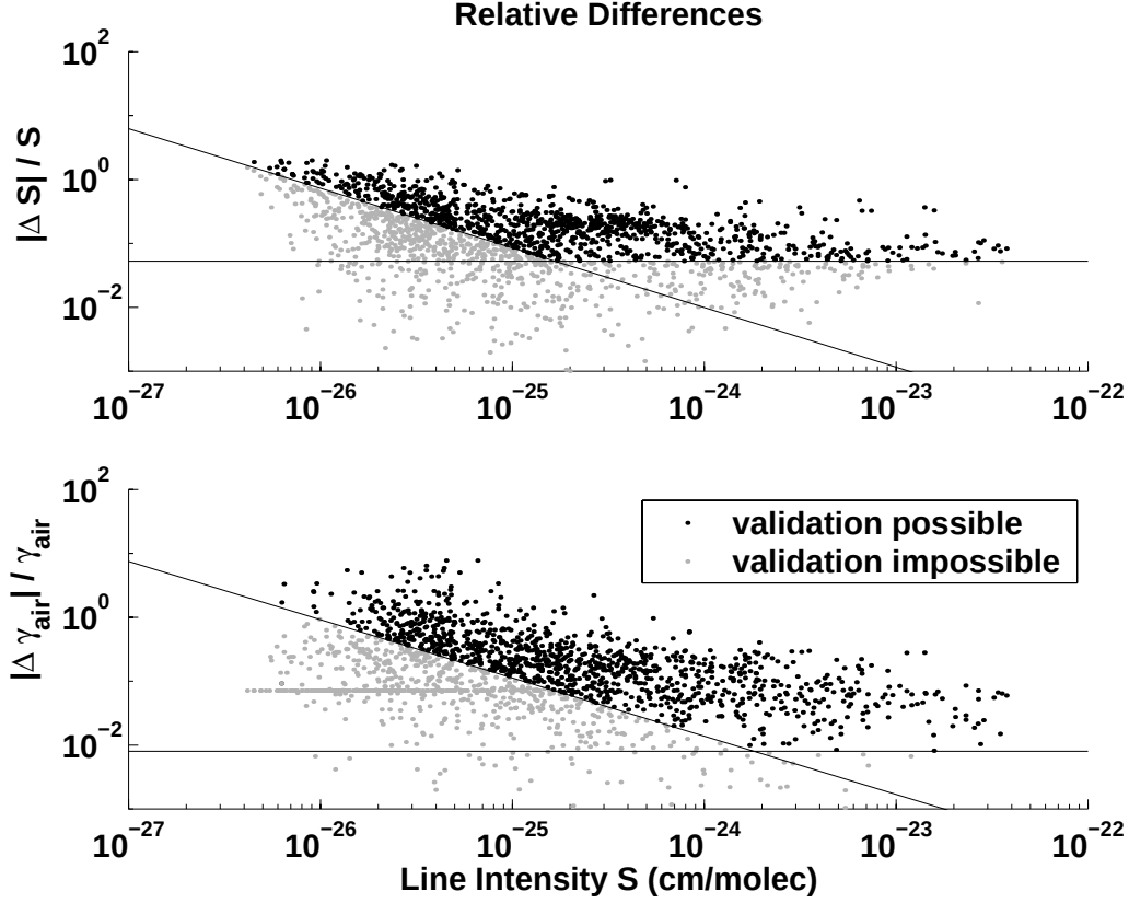
Figure 2.4: The amplitude of relative differences of line parameters |S_{\text{hit01}} - S_{\text{ulb04}}|/S_{\text{ulb04}} (upper graph) and |\gamma_{\text{air, hit01}} - \gamma_{\text{air, ulb04}}|/\gamma_{\text{air, ulb04}} (lower graph) given in HITRAN-2000 and ULB-UFR-BIRA. Line parameter differences that exceed the uncertainty of the ground-based measurement are shown as black dots. The other line parameter differences are shown gray. The solid lines are the same as in Fig. 2.2.
