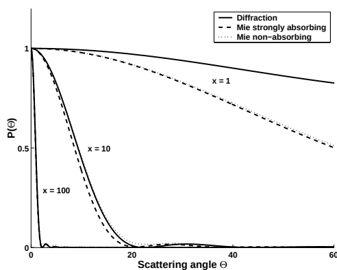
Figure 5.2: Phase function P(\Theta) for diffraction (solid) and Mie scattering by strongly-absorbing (dashed) and non-absorbing spheres (dotted). The intensity is normalized to 1 at \Theta = 0^\circ . The sizes of the spheres are given in terms of the size parameter x = 2\pi r/\lambda .
