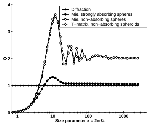
Figure 5.3: Scattering efficiency Q for diffraction (crosses), from Mie calculations for strongly absorbing spheres (solid circles) and non-absorbing spheres (empty circles), and from T -matrix calculations for non-absorbing spheroids (empty diamonds).
