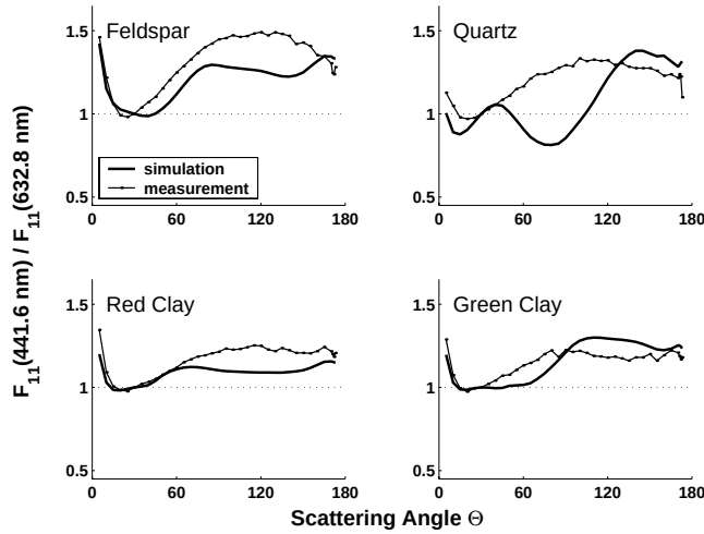
Figure 6.4: Ratio of the phase functions F_{11}(\Theta) at \lambda = 441.6 nm and F_{11}(\Theta) at \lambda = 632.8 nm. The ratio of phase functions is shown for measurements and simulations for various mineral dust samples. A priori estimates are used for the refractive index and the size distribution (case A).
