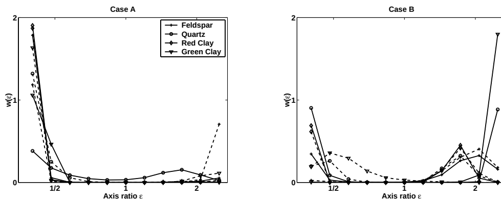
Figure 6.6: Aspect ratio distribution retrieved from the scattering matrices of the feldspar sample (crosses), the quartz sample (circles), the red clay sample (diamonds), and the green clay sample (triangles) measured at the wavelengths 421.6 nm (solid) and 632.8 nm (dashed). The left graph shows the results of a retrieval using a priori estimates for the refractive index and the size distribution (case A). The right graph shows results of a retrieval where all parameters are retrieved simultaneously (case B).
